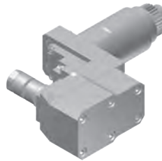
CCB730000 Slotting unit RATIO 1 : 0.75 RPM(MAX) 3000 SAW OD(MAX) Ø45mm SAW ARBOR SHANK Ø12.7mm
