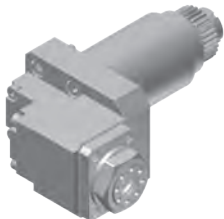
CCB761000 Cross drilling/milling unit RATIO 1 : 1 RPM(MAX) 3000 TOOL CLAMPING ER16
