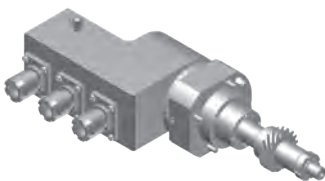
CCY496300 3 spindle drilling/milling unit RATIO 1 : 1 RPM(MAX) 6000 TOOL CLAMPING ER16M ANGLE ADJUSTMENT ±90°
