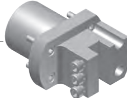
CCB611120 Turning tool holder TOOL SHANK Ø42.0mm BITE HOLDER SHANK 12x12mm
